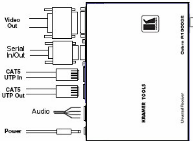
Figure 4: Cobra R1300S2 Universal Receiver Connections
